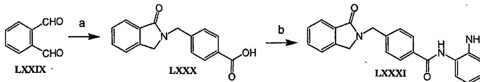
Scheme 16
